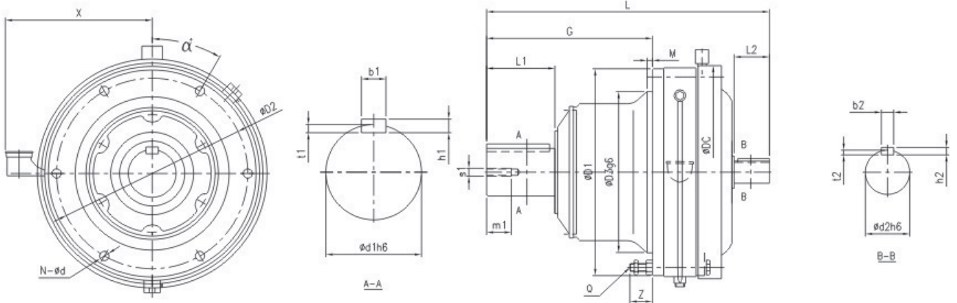
Installation Dimensions THF-613~THF-626
