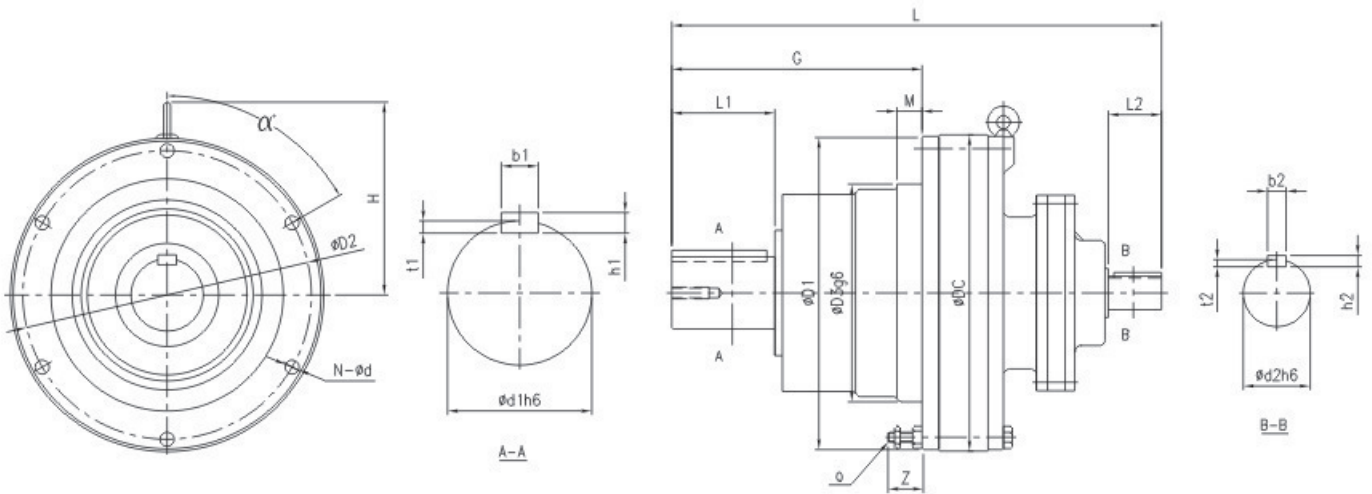
Installation Dimensions THF-613/08~THF-618/10
